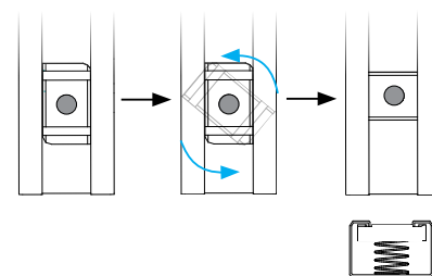
Fixes into Carrier Rail with M10 Spring Nut
