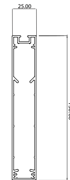
150mm x 25mm Baffle
