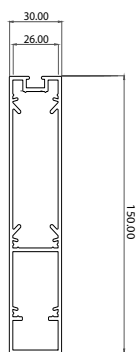
150mm Baffle
