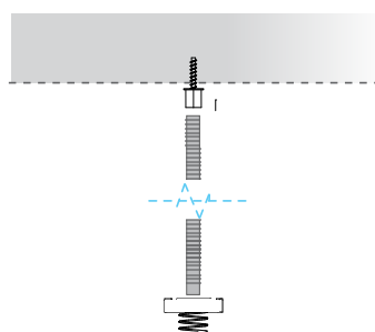
Threaded rod suspension system
