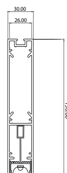
150mm Baffle with Gridlux
